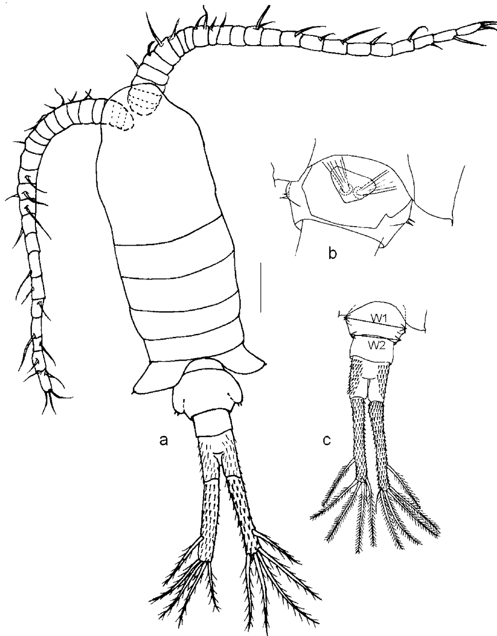
Fig. 3. Eurytemora caspica sp. nov., female, ZIN 55060 (holotype): a – habitus, dorsal view; b – genital double-somite, ventral view; c – uropod, ventral view. Scale bar: a, b – 200 \mu m; c – 100 \mu m.
