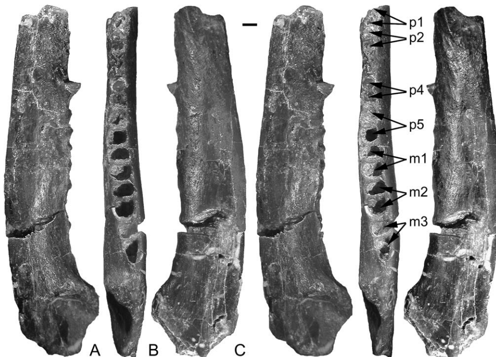
Fig. 7. “Zhelestidae” indet., unnamed large sp. A. Locality SSHD-8 (early Cenomanian), Khodzhakul Formation, Sheikhdzheili local fauna, Kyzylkum Desert, Uzbekistan. A–C, CCMGE 1/11658, stereo-photographs, left dentary with alveoli for p1-2, 4-5, m1-3: A, labial, B, occlusal, and C, lingual views. Scale bar represents 1 mm.
