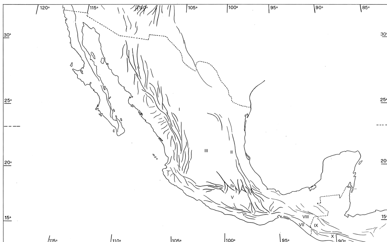
FIGURE 9. Main orographic formations of Mexico. Original map prepared by Violeta Halffter and used on many occasions in the biogeographic studies of the Mexican Transition Zone. I, Sierra Madre Occidental; II, Sierra Madre Oriental; III, Mexican Plateau; IV, Trans-Mexican Volcanic Belt; V, Balsas Basin; VI, Sierra Madre del Sur; VII, Sierra Madre de Chiapas; VIII, Chiapas Highlands; IX, Guatemalan Plateau; X, Central American Nucleus.
