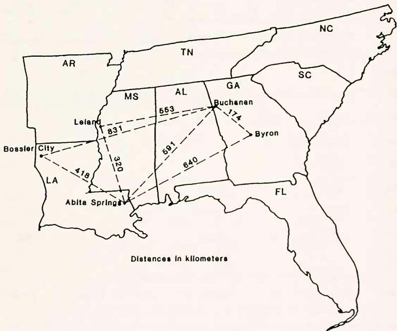
Figure 1. Map of Southeastern United States showing release sites (Byron, GA, Leland MS, and Bossier City, LA) and recovery sites (Buchanan, GA and Abita Springs LA) of Harmonia axyridis and the straight-line distances (KM) between sites.
