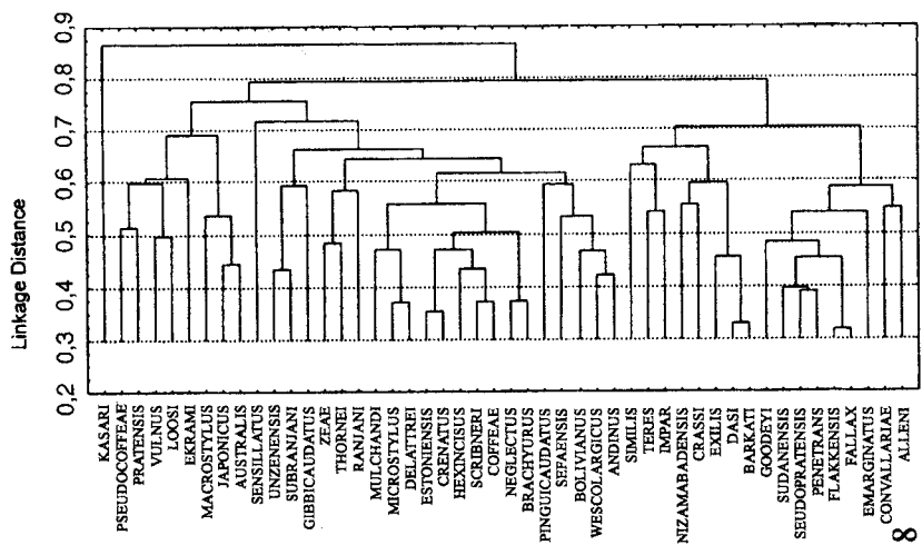
Figs 7-9. Dendrograms of the cluster tree analysis of the morphological similarity of the genus Pratylenchus prepared in the STATISTICA package. 7: UPGMA linkage with Pearson r as the distance measure; 8: UPGMA linkage with Euclidean distances. 9: Ward's method linkage with Euclidean distances.
